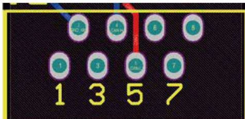
CAN Port
